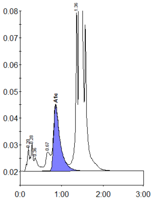
Peak table - ID: 10480537
